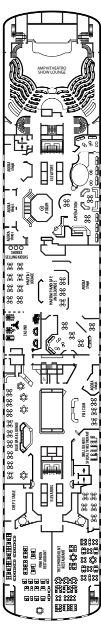
DECK 8
